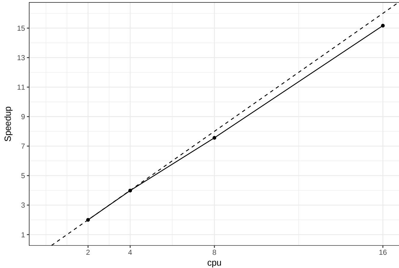
Speedup vs 1 core
